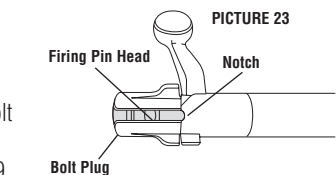
Bolt in Cocked Position
